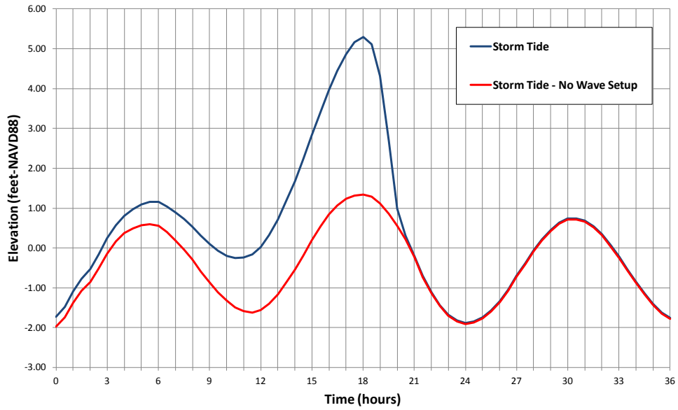
Martin County 15 -Year Hydrograph
