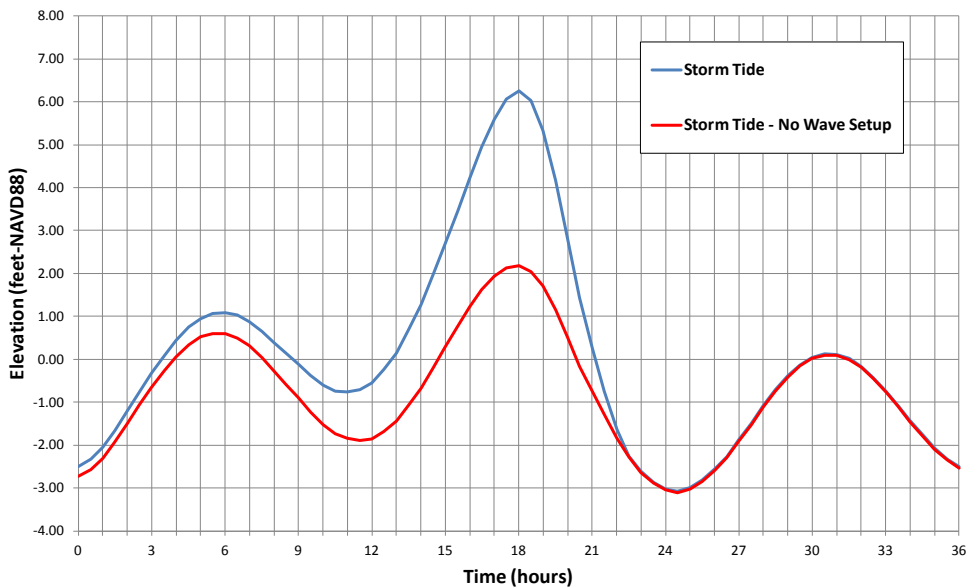
Martin County 25 -Year Hydrograph
